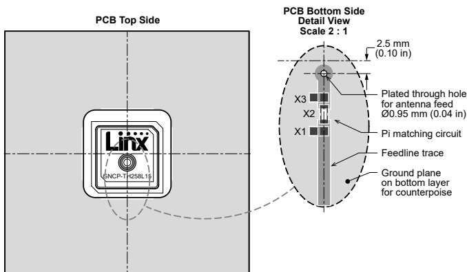
Figure 15. Recommended PCB Layout for the ANT-GNCP-TH258L15
