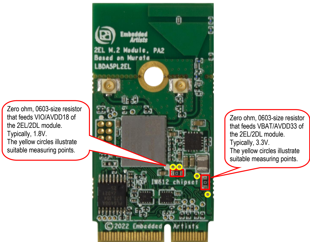
Figure 8 – Current Measurement
