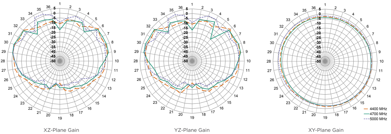
Figure 16. Radiation Patterns for ANT-5GW-IPW2-NP, Center of Ground Plane
