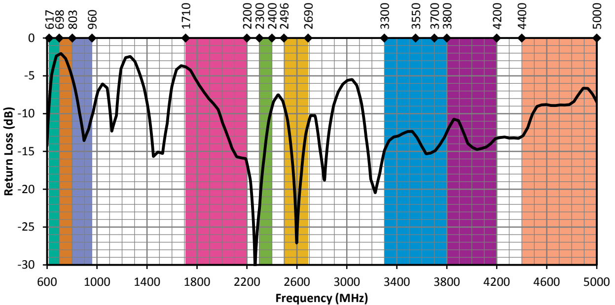
Figure 5. ANT-5GW-IPW2-NP Return Loss, Free Space
