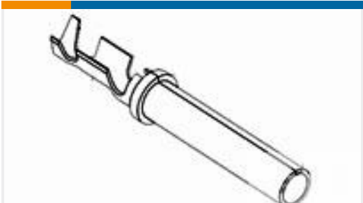
TE Part #776493-2 SOC, SF, SIZE 16, 18-20 AWG, NI/SN
