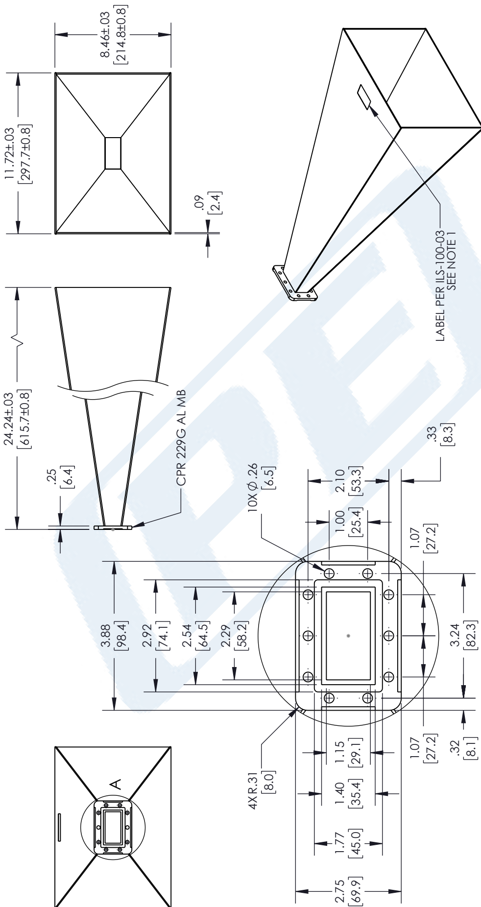
DETAIL A
