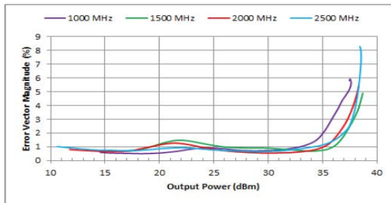
Error Vector Magnitude (%) [w/ QPSK Waveform]
