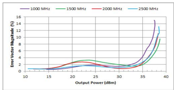
Error Vector Magnitude (%) [w/ 64QAM Waveform]
