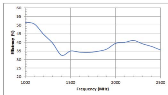
Efficiency
