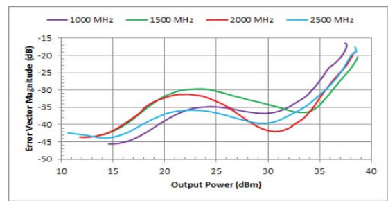
Error Vector Magnitude (dB) [w/ 64QAM Waveform]
