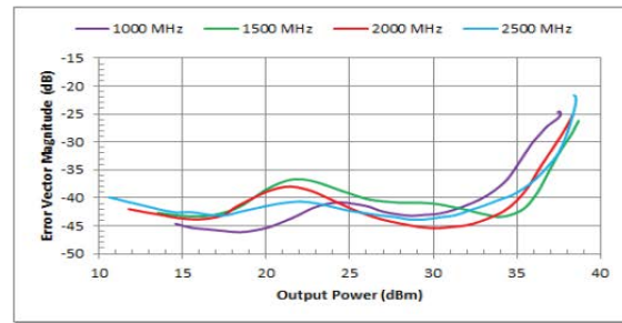
Error Vector Magnitude (dB) [w/ QPSK Waveform]
