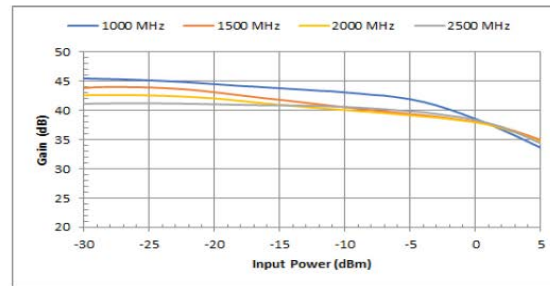
Gain vs. Input Power
