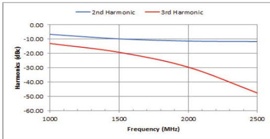
Harmonics (@ Psat)
