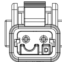
KEY-D CONFIGURATION ATMH06-2SD TPA COLOR: BROWN
