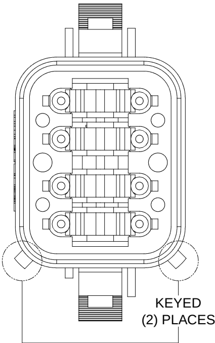
P/N AT06-08SB-RD01 KEY-B CONFIGURATION STANDARD COLOR: BLACK
