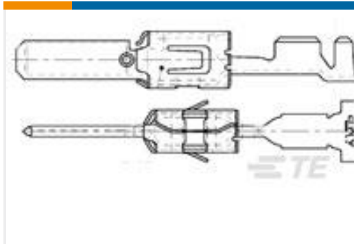
TE Part # 185028-1 TAB F 2.8x0.8 CONTACT CS SWS Sn
