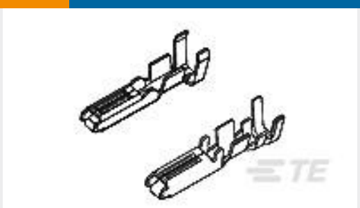
TE Part # 345208-1 070 SERIES RECEPT.
