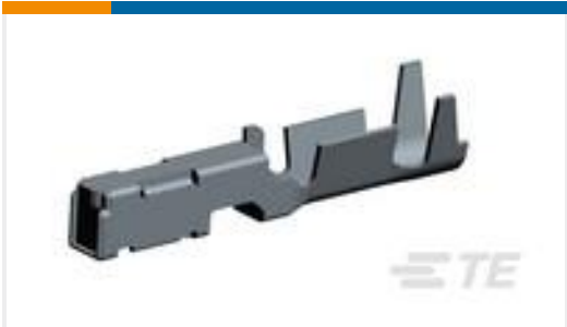
TE Part # 1924955-3 CONTACT,FEMALE0.64,20-22AWG, UNSEAL
