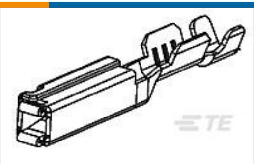
TE Part # 1393367-2 GET-SOCKET TERMINAL, SILVER VE
