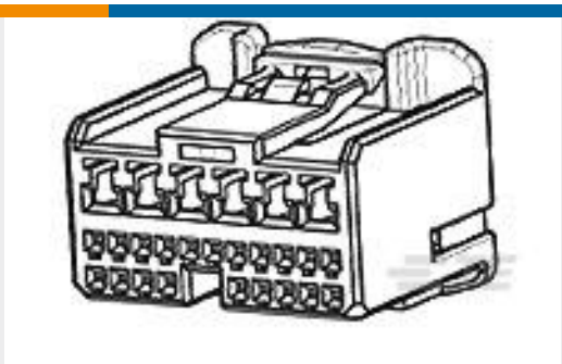
TE Part # 1318756-2 025/090 ECU PLUG HSG ASSY 24P
