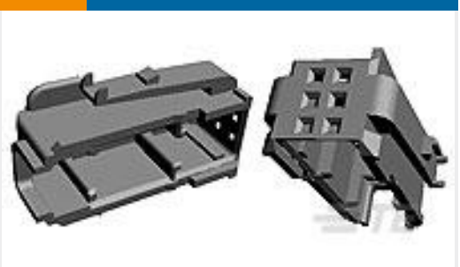
TE Part # 953382-2 COVER FOR 6W HSG MQS GEN2
