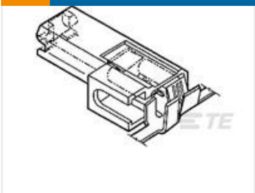
TE Part #1969106-2 ULTRA-POD 187 ASSY REC 22-16 AWG TPBR
