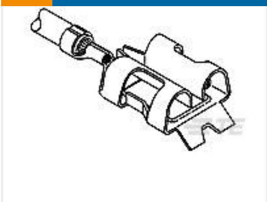
TE Part #640748-7 HEAVY DUTY BURNER REC 18-14 AWG PHBRZ
