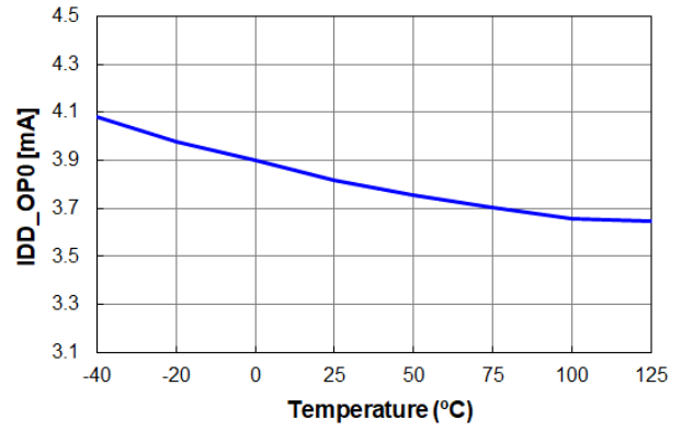
Figure 16. I DD-OP0 vs. Temperature
