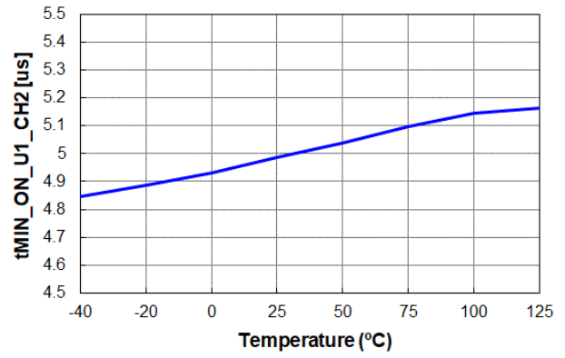
Figure 6. t_{\text{MIN-ON-U1-CH2}} vs. Temperature
