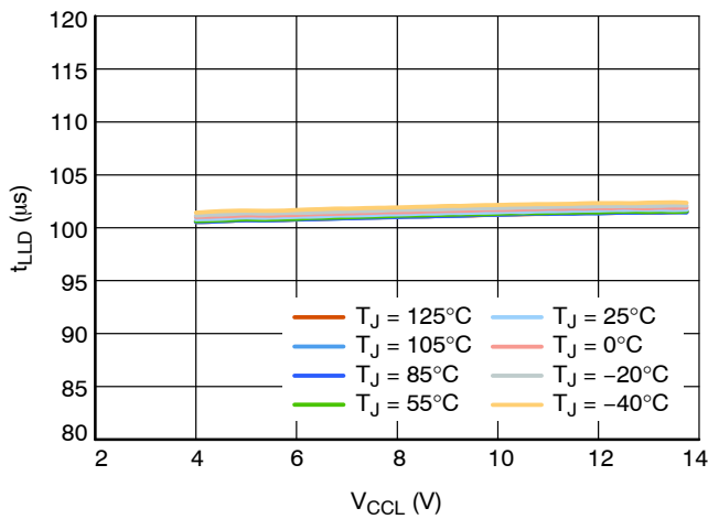
Figure 42. Light Load Detection Time t_{LLD} = 100 \text{ μs}
