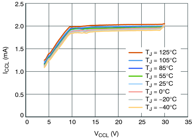
Figure 16. VCCL Current Consumption for 10 V Driver, V_{CS} = -1 to 4 V, f_{CS} = 100 kHz, C_{DRV} = 1 nF
