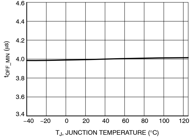
Figure 39. Minimum Off-time t_{OFF\_MIN} = 4 \text{ μs}
