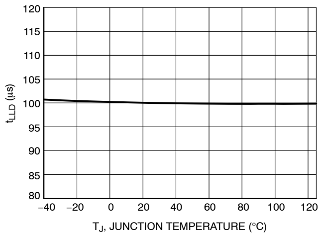
Figure 43. Light Load Detection Time t_{LLD} = 100 \text{ μs}
