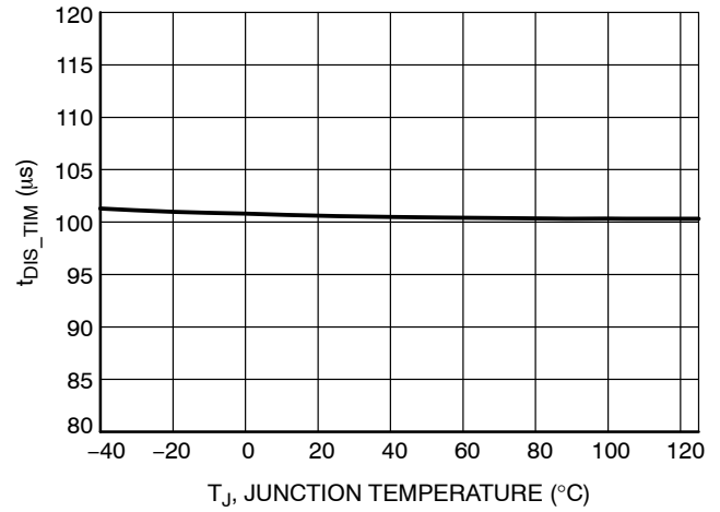
Figure 35. Delay to Disable Mode, V_{TRIG} = 5 V
