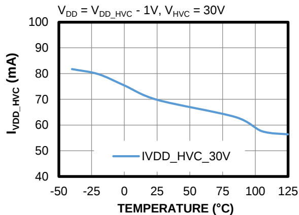
VDD Maximum Charging Current vs. Temperature V_{DD} = V_{DD\_HVC} - 1V, V_{HVC} = 30V
