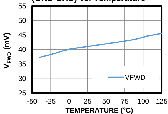
Forward Regulation Voltage (GND-SRD) vs. Temperature
