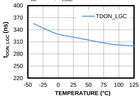
Turn-On Delay during LGC Mode
