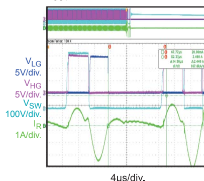
Capacitive-Mode Protection
