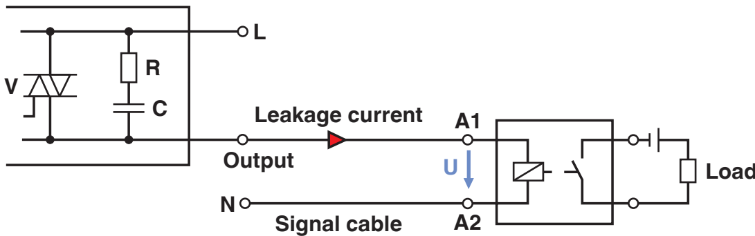
Application drawing
