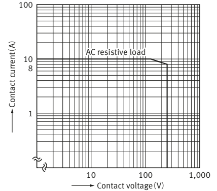
1-3. Max. switching capacity ( Inrush/reinforced insulation type: 1 Form A )
