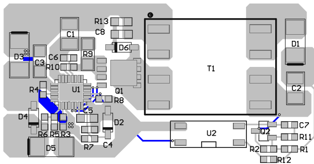
Figure 9: Recommended Layout
