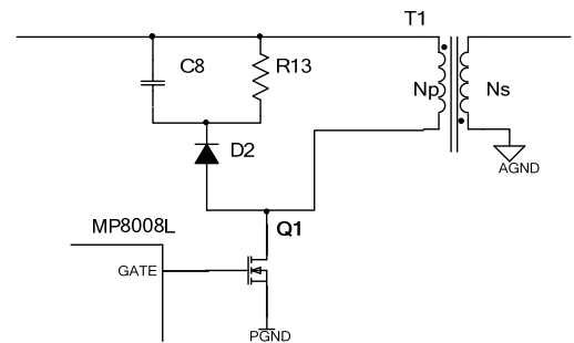
Figure 8: RCD Snubber
