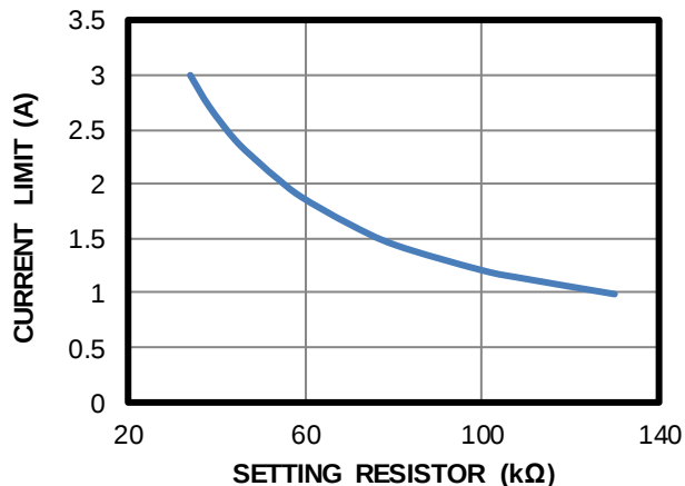
Switching Current Limit vs. Setting Resistor
