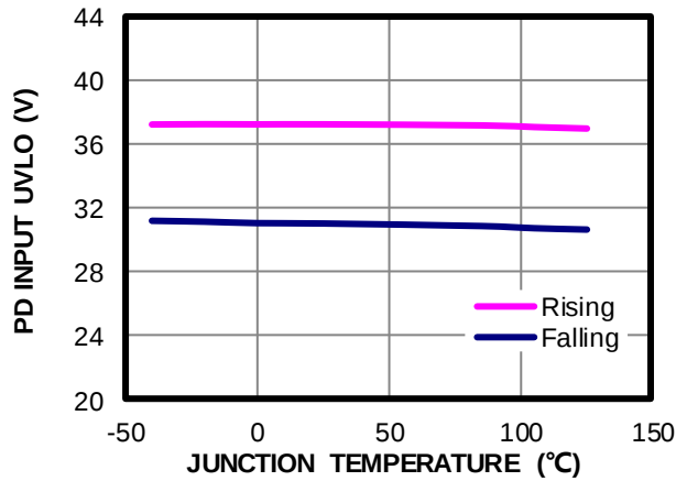
PD Input UVLO vs. Junction Temperature
