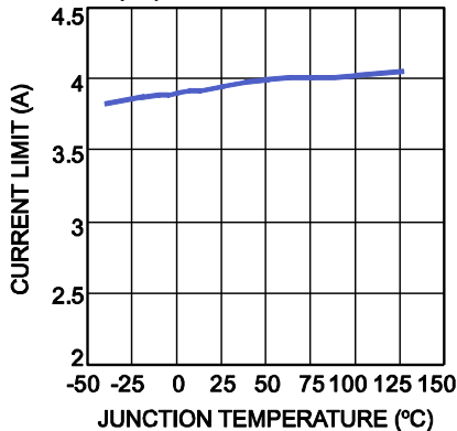
DC Converter Current Limit vs. Temperature
