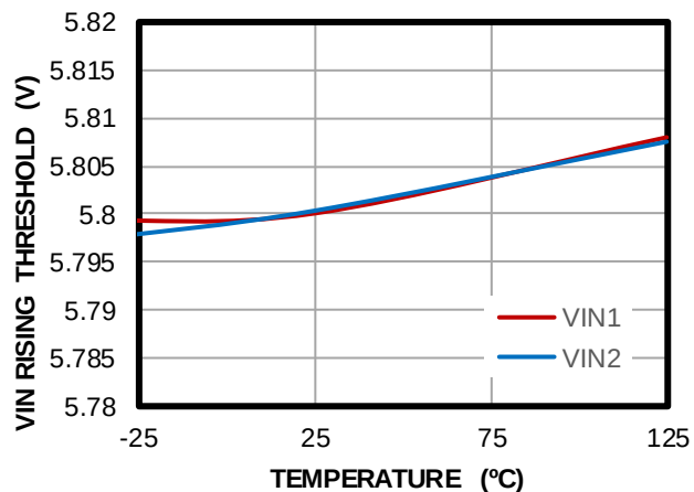
V IN Rising Threshold vs. Temperature
