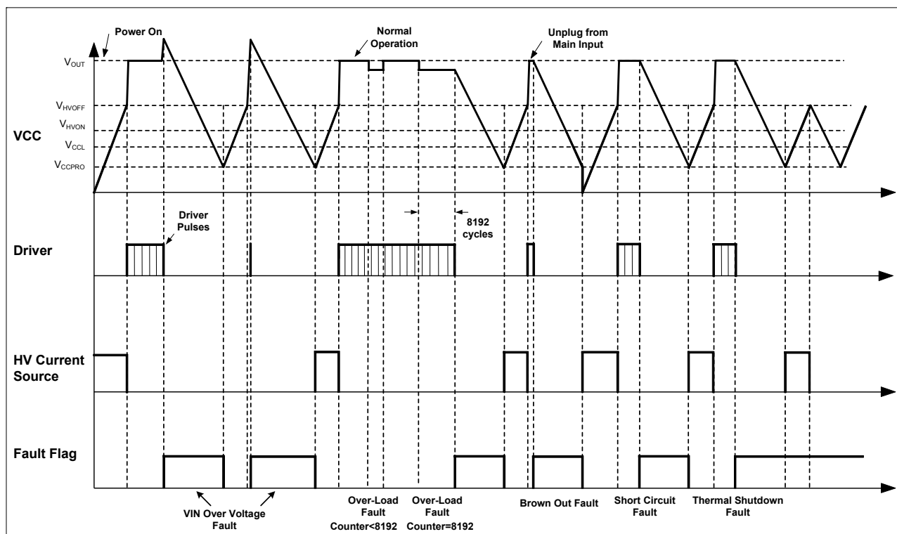
Figure 9: Signal Evolution in the Presence of a Fault
