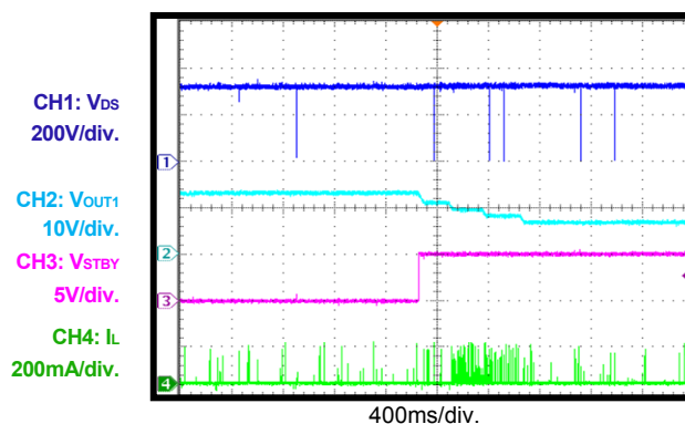
Standby Entry No Load
