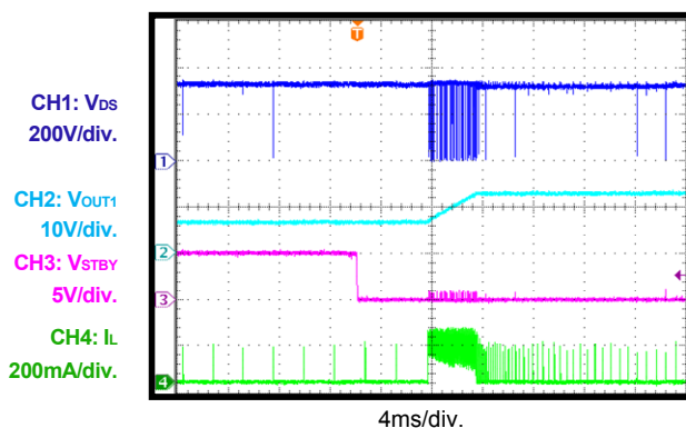
Standby Recovery No Load
