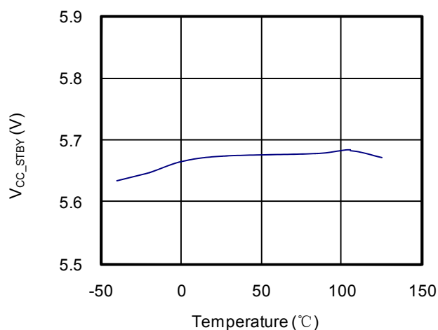
V_{\text{CCSTBY}} vs. Temperature
