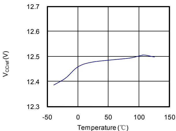
V_{\text{CCREF}} vs. Temperature
