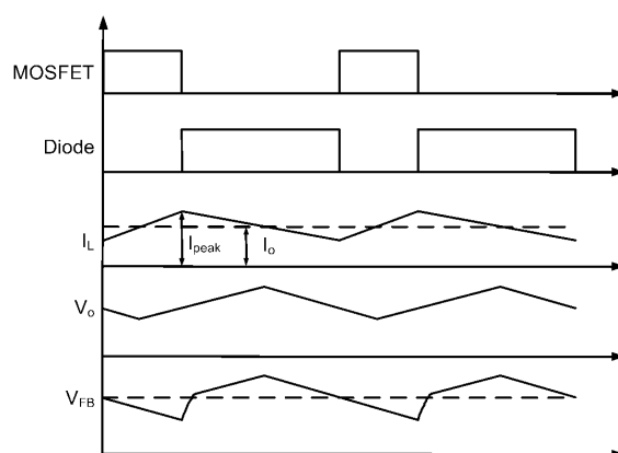
Figure 3: Constant Voltage Regulation
