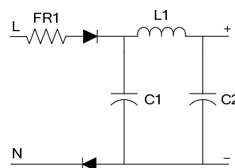
Figure 6: Half-Wave Rectifier
