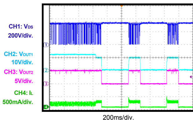
V_{OUT1} OLP Full Load
