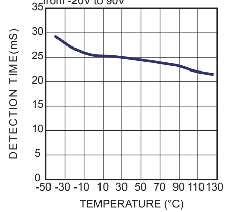
Detection Time vs. Temperature Chart
