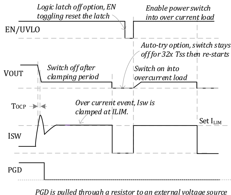
Fig. 39 - Over-Current Protection
