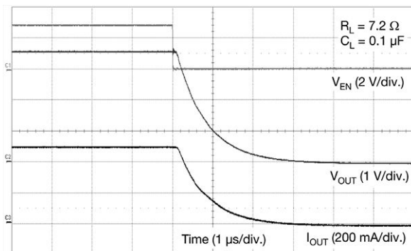
Fig. 23 - Turn-Off ( V_{IN} = 3.6\text{ V} )
