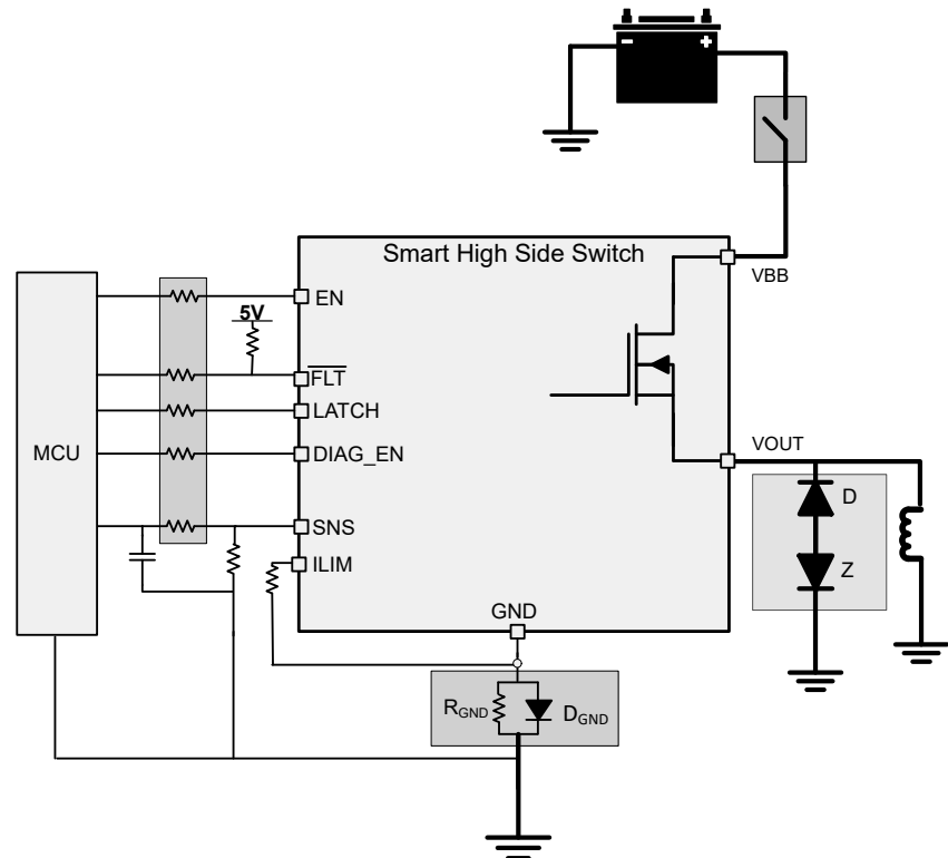
Figure 8-21. Loss of Battery
