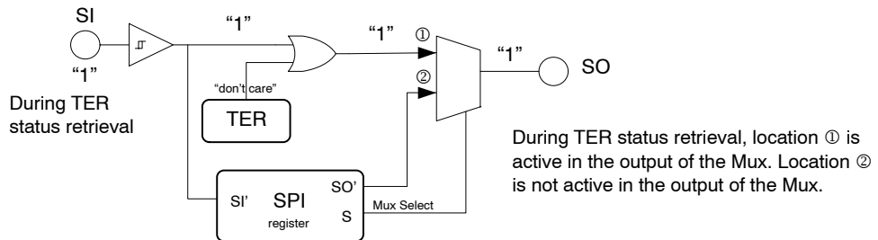
Figure 28. TERC False Reporting
