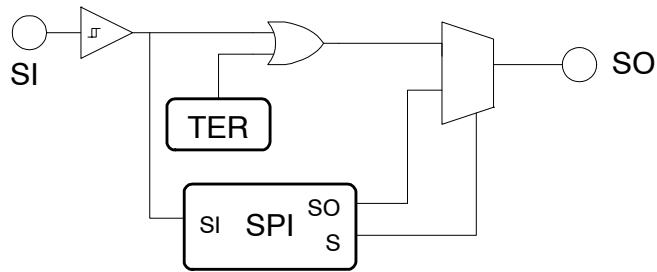
Figure 25. TERC SPI Link
