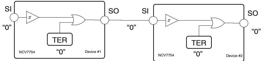
Figure 26. TERC (no error)
