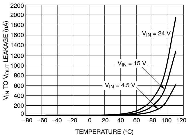
Figure 10. Input to Output Leakage vs. Temperature (EN = 0)
