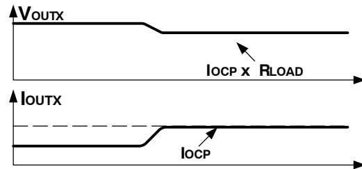
Figure 5. Overload
