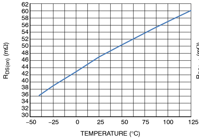
Figure 6. R_{DS(on)} ( m\Omega ) vs. Temperature ( ^{\circ}C ) at 3.3 V, I_{OUT} 100 mA
