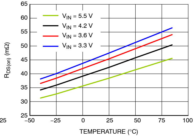
Figure 7. R_{DS(on)} ( m\Omega ) vs. Temperature ( ^{\circ}C ), I_{OUT} 2 A
