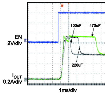
Inrush Current with Different Load Capacitance R_L=11\Omega , Start up by EN
