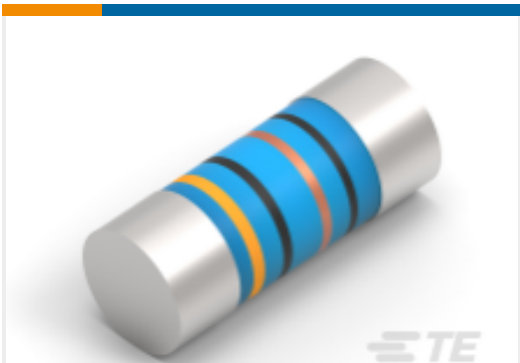
TE Part #2-2176316-2 MELF SMA_A 5K6 0.1% 15PPM 0207 1W
