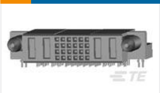
TE Part #1-6450160-0 MBXL R/A RCPT 2P+24S+2P
