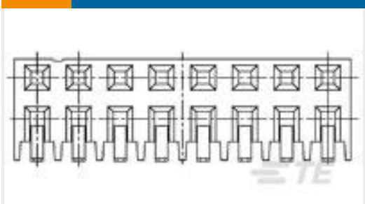
TE Part #1734606-6 AMPMODU, 2mm Pitch, 6P, R/A SMT, 8Au"
