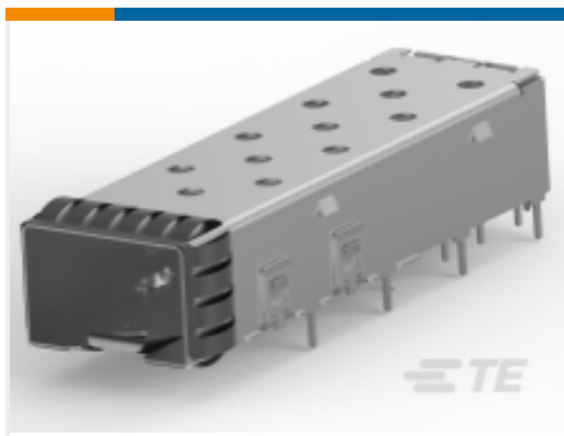
TE Part # 2110304-1 SFP+ 1x1 Cage Assembly, Solder Tail
