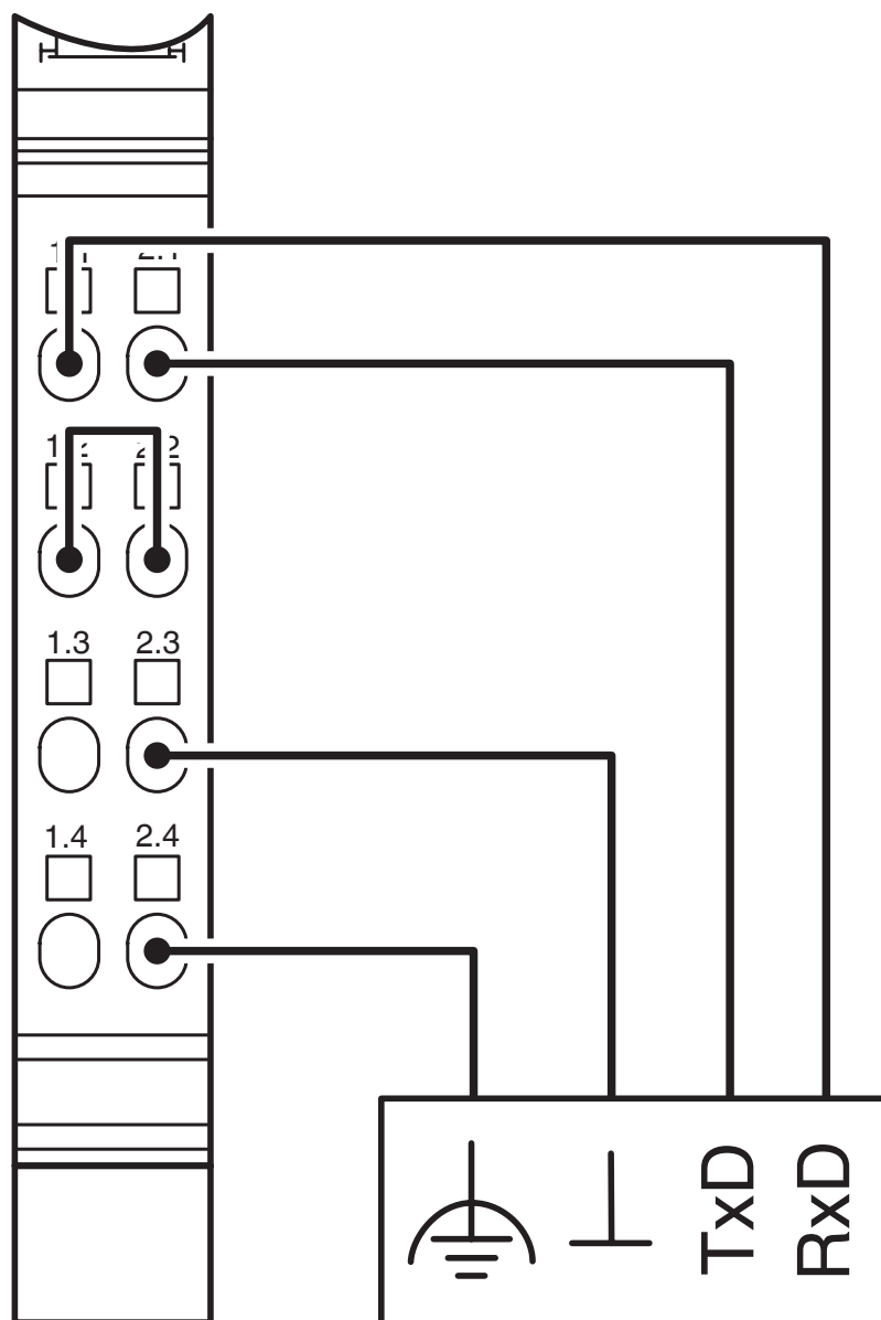
Connection diagram
