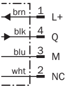
Light switching
