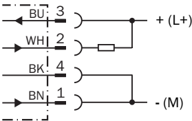
NPN dark-switching
