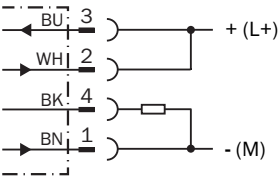
PNP dark-switching
