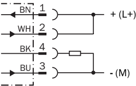
PNP light-switching
