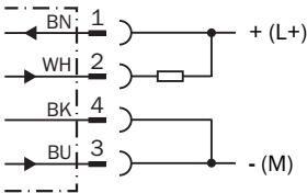
NPN light-switching
