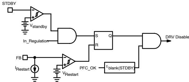
Figure 21. Standby Circuit Block
