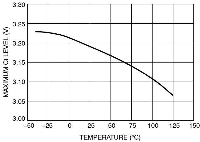
Figure 5. Maximum C_t Level ( V_{CTMAX} ) vs. Temperature
