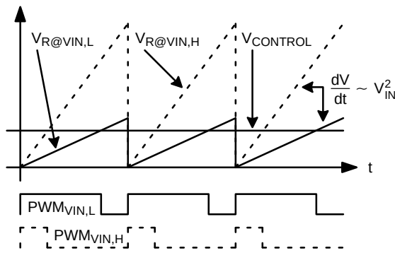
Figure 10. Input-Voltage Feedforward
