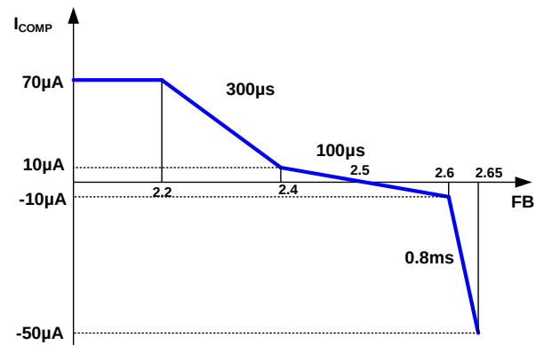
Figure 3: Nonlinear G_M
