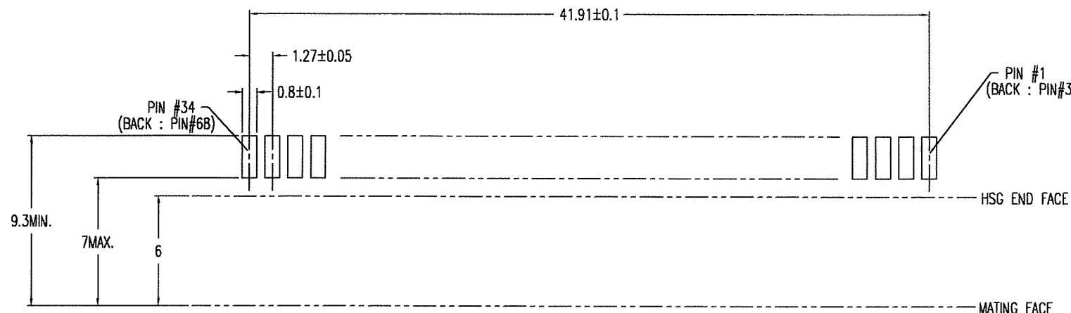
RECOMMENDED PWB FOOT PRINT LAYOUT
