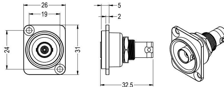
CP30125 - XLR 50Ω INSULATED BNC BLACK METAL FT Scale 2x1
