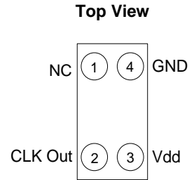
Figure 1. Pin Assignment
