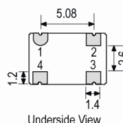
Underside View
